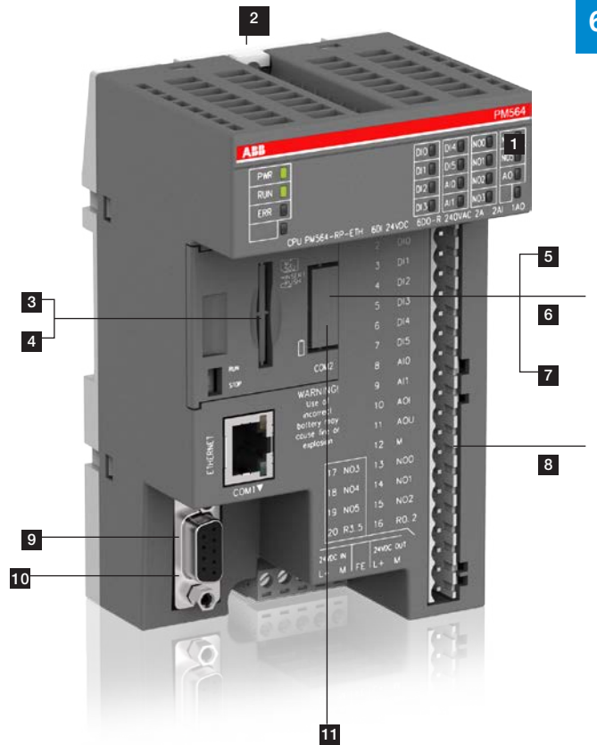
5 Adapter with realtime clock
